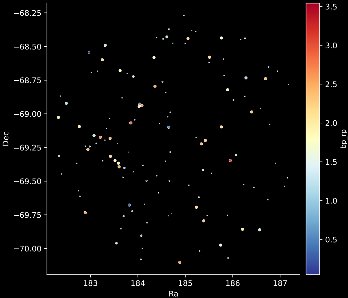
APOGEE DR17 Field: [279-31-O] Stars: 125
