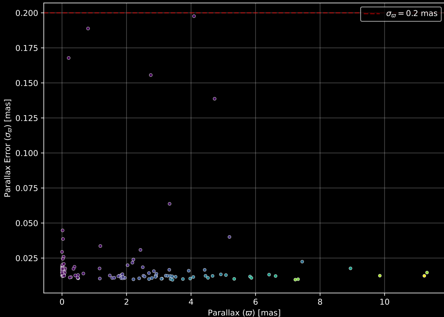
APOGEE DR17 Field: [279-31-O] Parallax Quality (n= 125)
