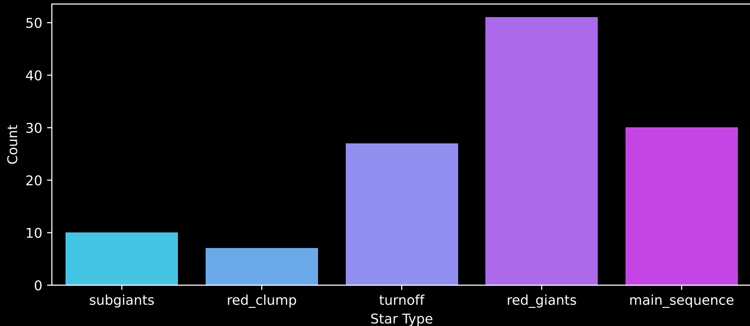
APOGEE DR17 Field: [279-31-O] Count plot of Star Type
