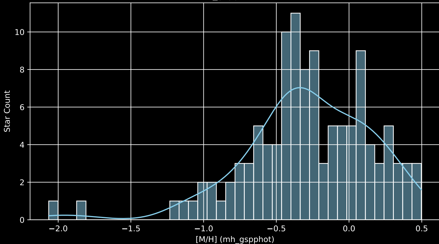
APOGEE DR17 Field: [279-31-O [M/H] (mh_gspphot) (n= 117)
