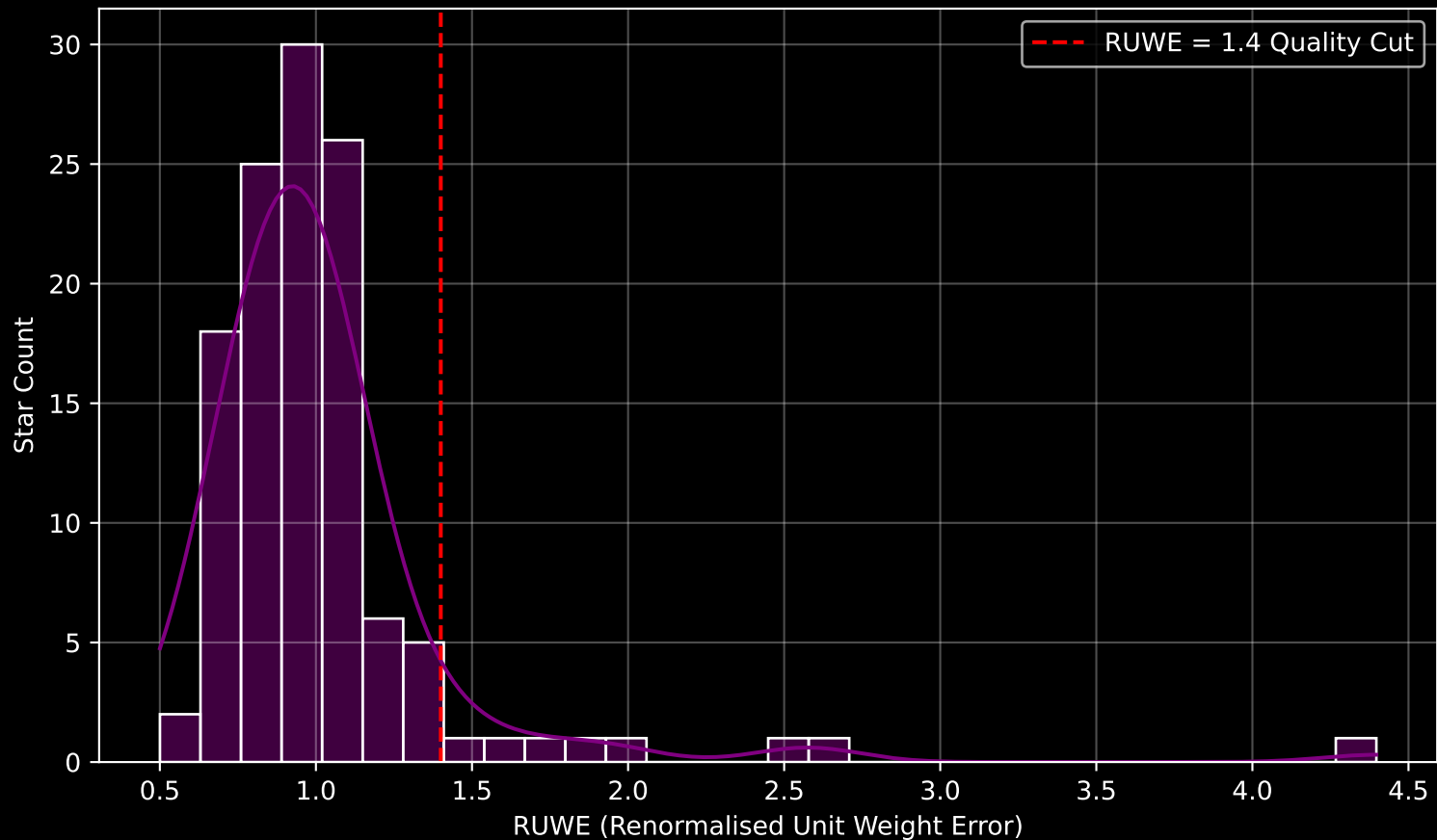
GAPOGEE DR17 Field [279-31-O] RUWE Distribution (n= 120)
