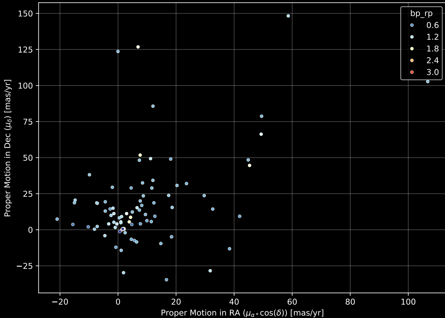
APOGEE DR17 Field: [279-31-O] Proper Motion Diagram (n= 125)
